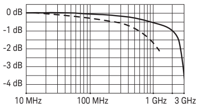
插入损耗
