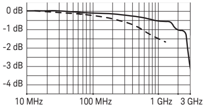
插入损耗
