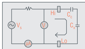
图4.2；测试回路开路 C_m = C_c * C_x / (C_c + C_x) \ll C_x
