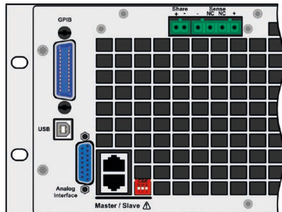
带3W选项型号的后板连接器 / Rear connectors of models with option 3W
