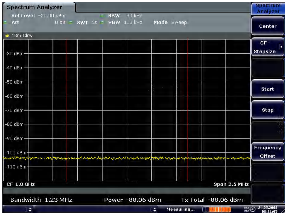
Figure 6-30: Measurement of the R&S ESRP's intrinsic noise power in a 1.23 MHz channel bandwidth.
