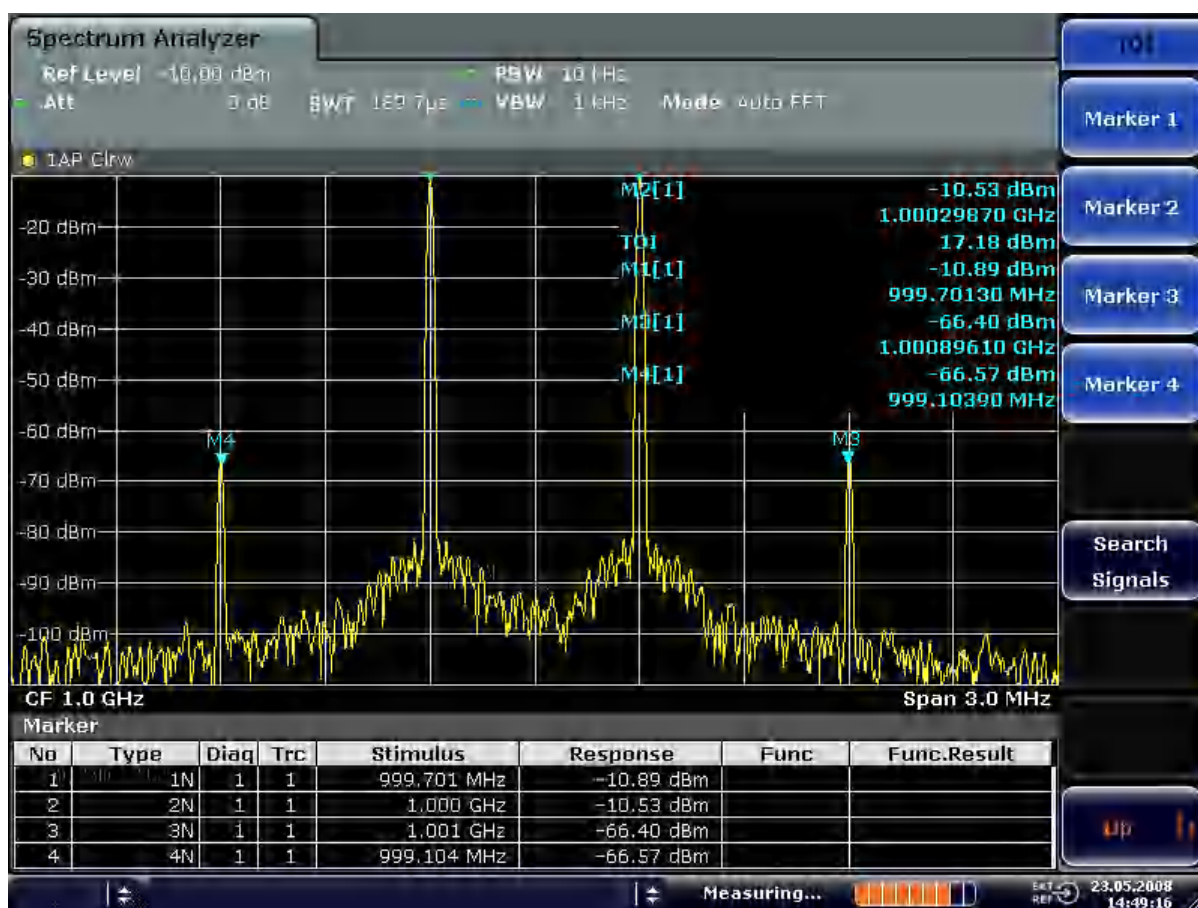
Figure 6-24: Result of intrinsic intermodulation measurement on the R&S ESRP.
