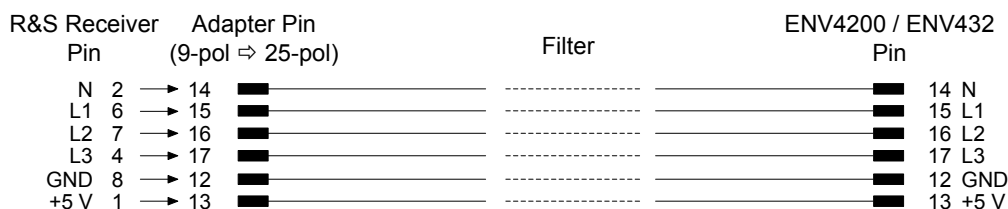
Figure 5-8: Connection from R&S ESRP to R&S ENV4200 or R&S ENV432
