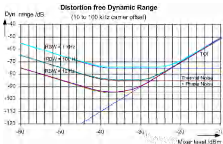
Figure 6-12: Intermodulation-free dynamic range of the R&S ESRP as a function of level at the input mixer and of the selected resolution bandwidth
