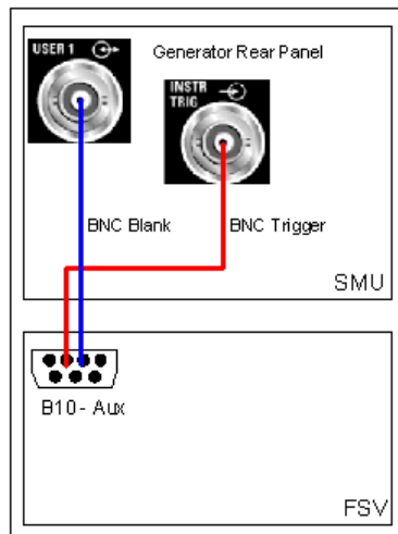
Figure 8-1: TTL connection for an SMU generator
