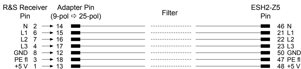
Figure 5-5: Connection from R&S ESRP to R&S ESH2-Z5
