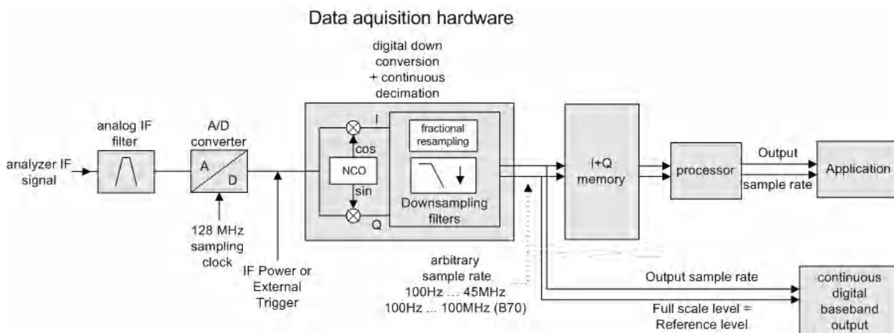
Figure 7-1: Block diagram illustrating the R&S ESRP signal processing
