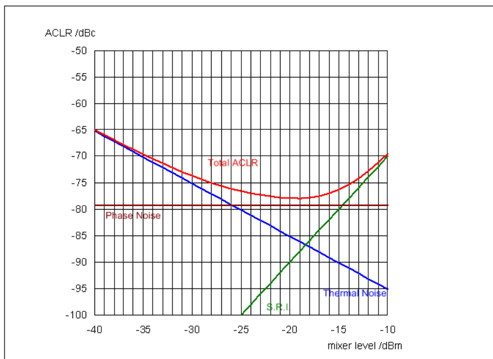
Figure 6-35: The R&S ESRP's dynamic range for adjacent channel power measurements on W-CDMA uplink signals is a function of the mixer level.
