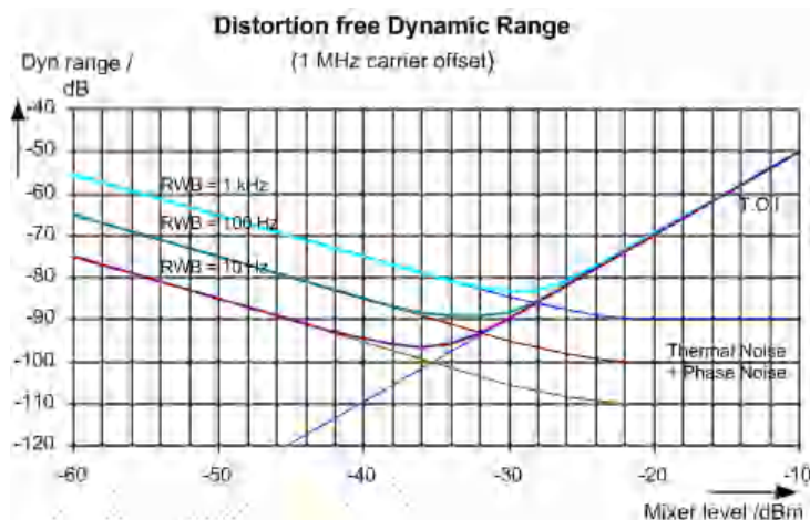
Figure 6-11: Intermodulation-free range of the R&S ESRP as a function of level at the input mixer and the set resolution bandwidth
