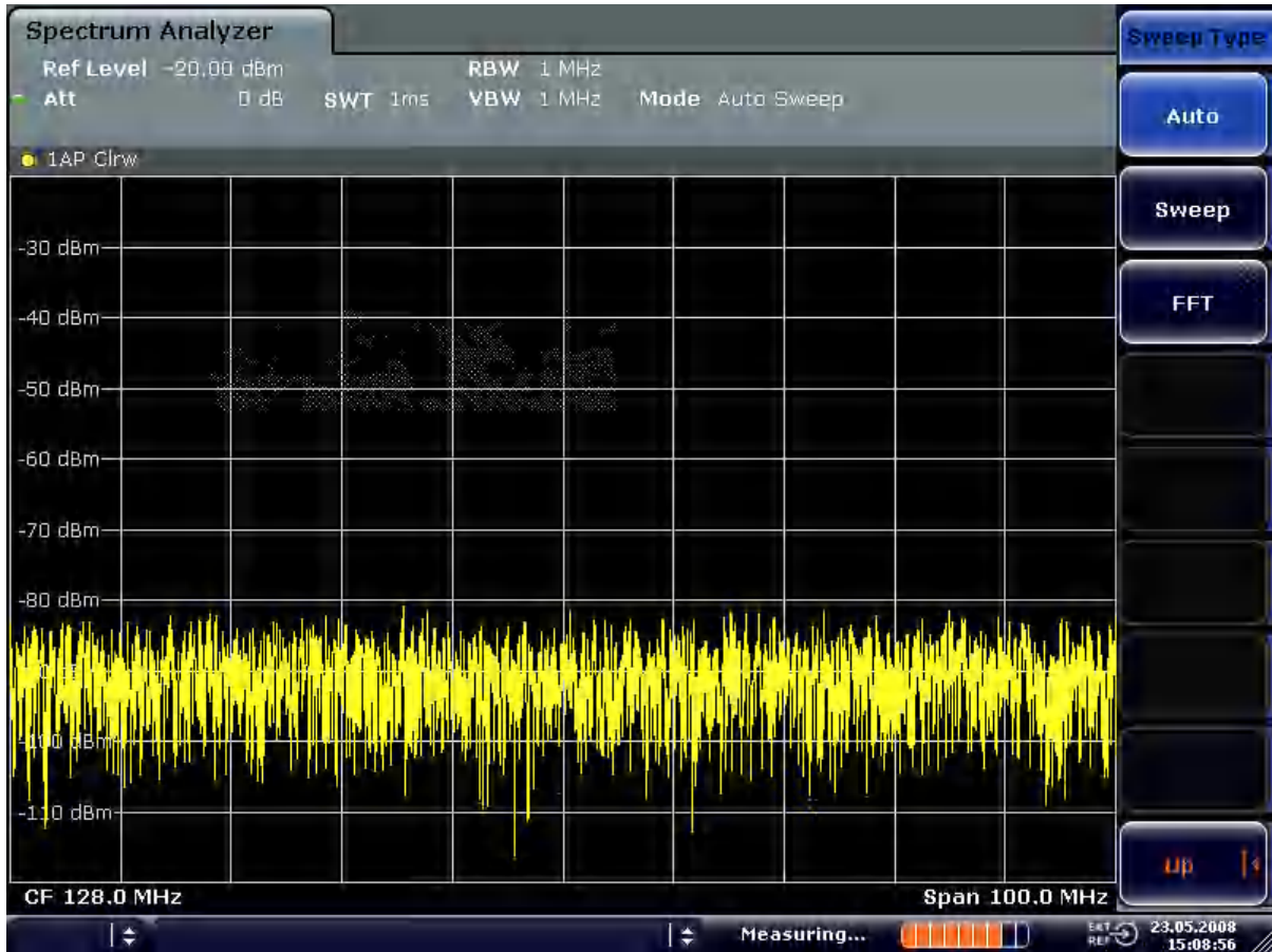
Figure 6-25: Sine wave signal with low S/N ratio. The signal is measured with the auto peak detector and is completely hidden in the intrinsic noise of the R&S ESRP.
