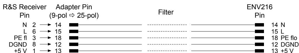
Figure 5-7: Connection from R&S ESRP to R&S ESH216
