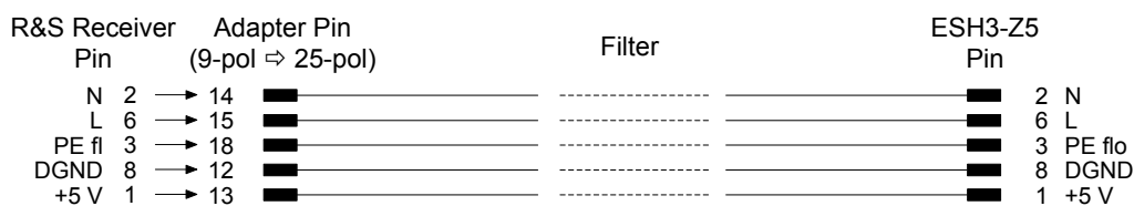
Figure 5-6: Connection from R&S ESRP to R&S ESH3-Z5
