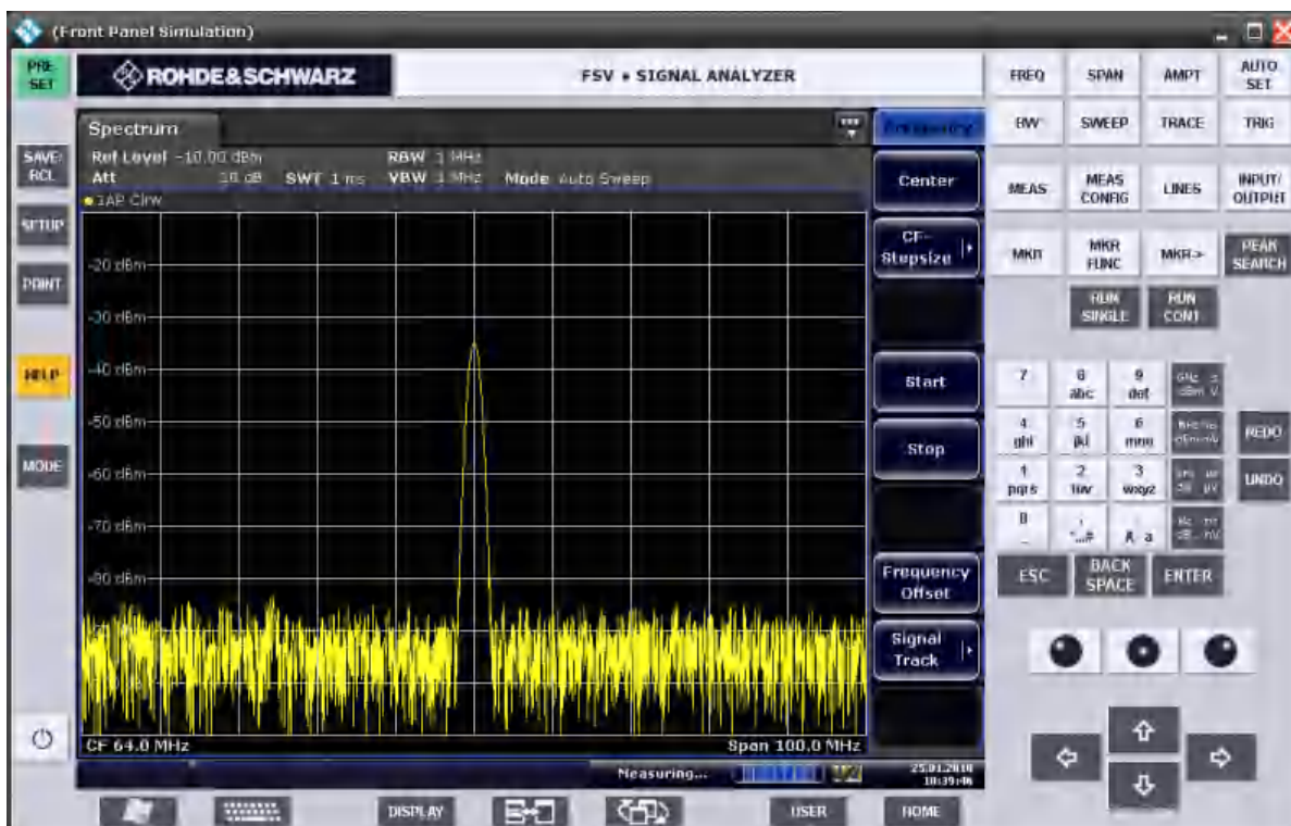
Figure 9-1: Soft frontpanel
