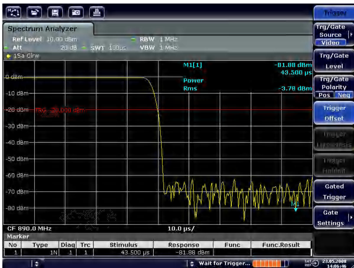
Figure 3-17: Falling edge of the GSM burst displayed with high time resolution
