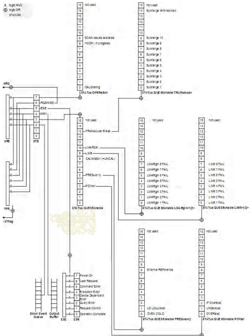
Figure 11-3: Overview of status registers in receiver mode
