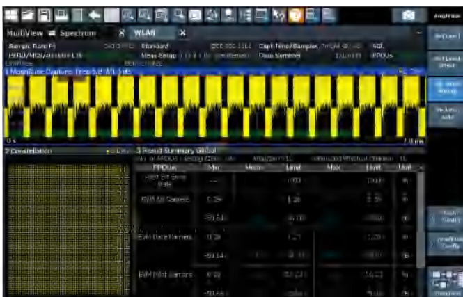
Analysis of a 320 MHz wide and 4096QAM modulated WLAN 802.11be signal using the R&S®FSW-K91BE option
