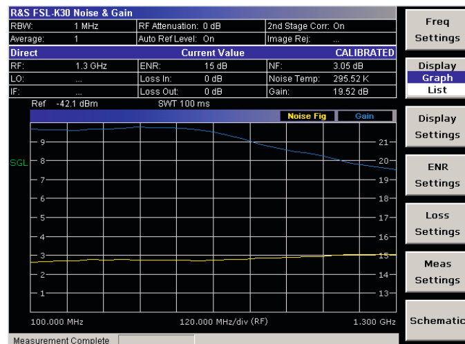
Measurements on an amplifier.
