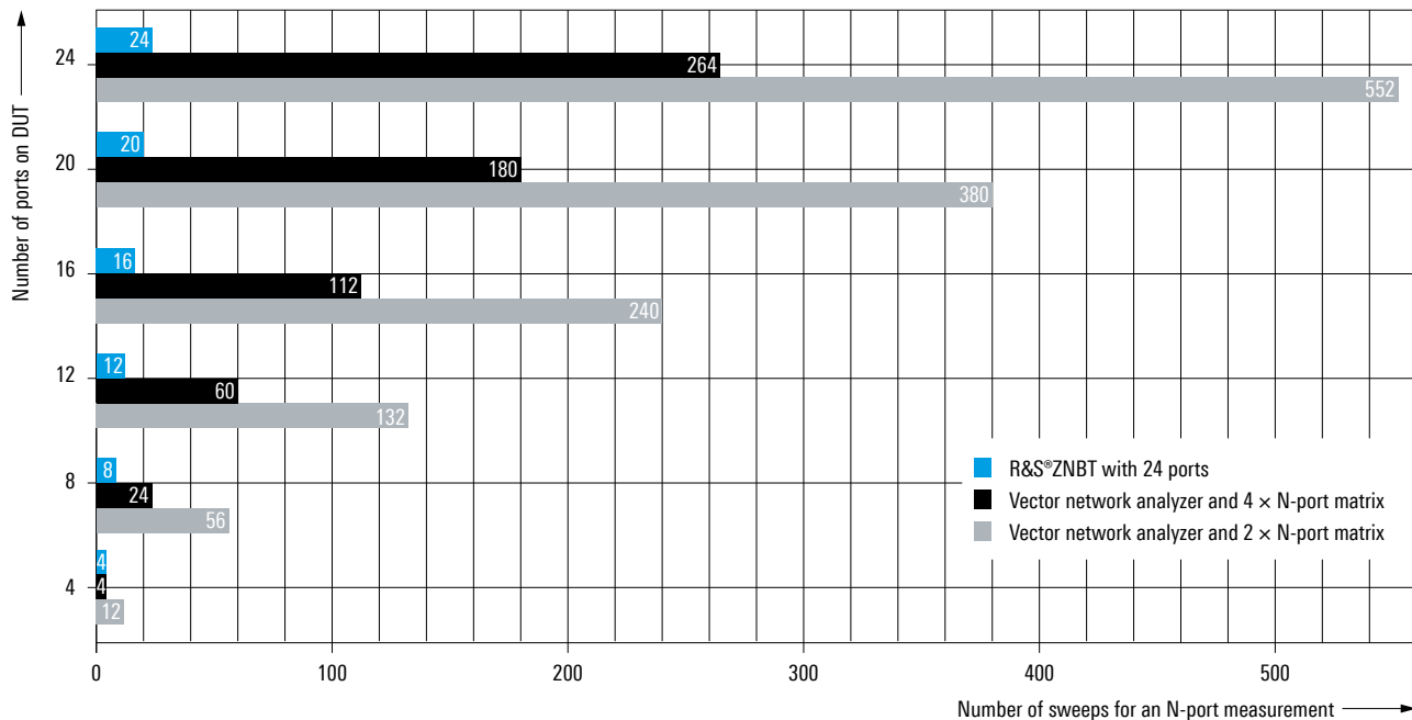
Comparison of measurement time: the R&S®ZNB T versus switch matrix based multiport solutions
