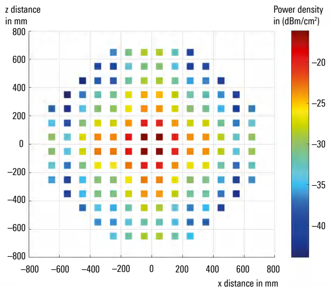
Average power density, base station 1, LTE, FDD, HPO, 3400 MHz
