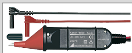
Kelvin Probes KC27
