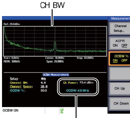
Channel power and OCBW power results
