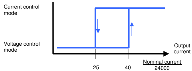
Fig. 3 Switching hysteresis between current and voltage control
