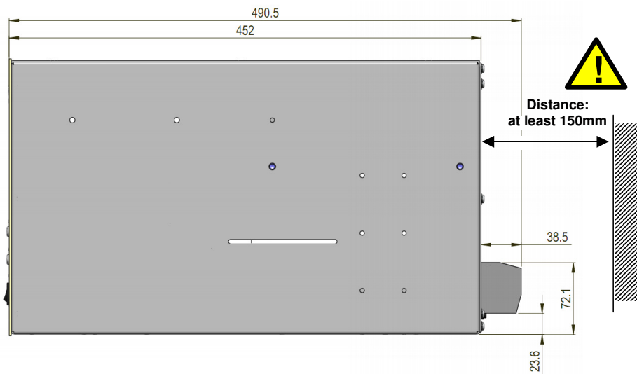
Fig. 12 Dimensions, side
