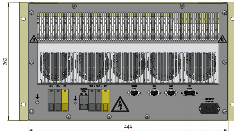
Fig. 11 Dimensions, rear
