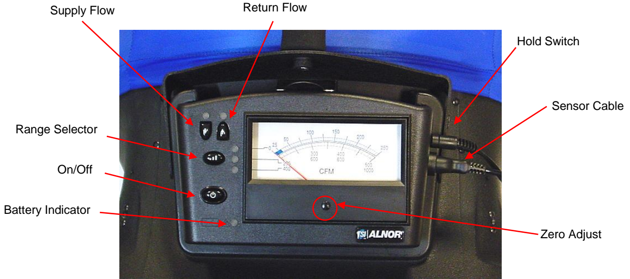
Figure 7 Analog Meter Components
