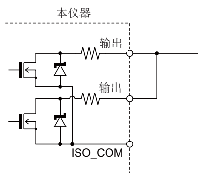
Wired OR
