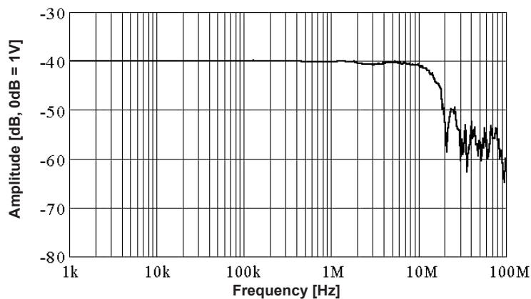
Figure 1 Frequency Characteristics (Typical Characteristics)
