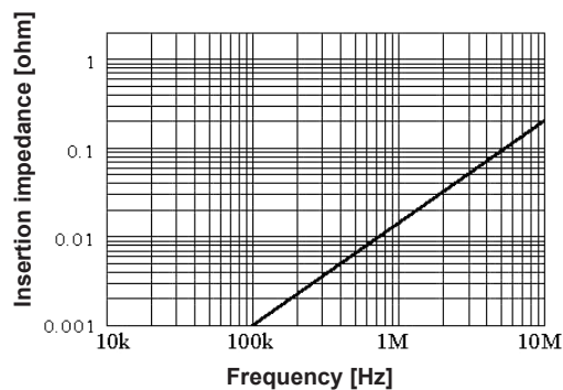
Figure 3 Insertion Impedance (Typical Characteristics)
