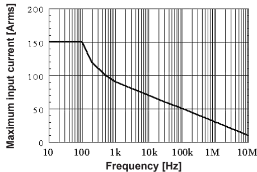
Figure 2 Derating According to Frequency
