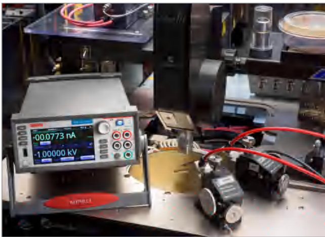
Characterize transistors with multiple SMU instruments on wafer or packaged transistors
