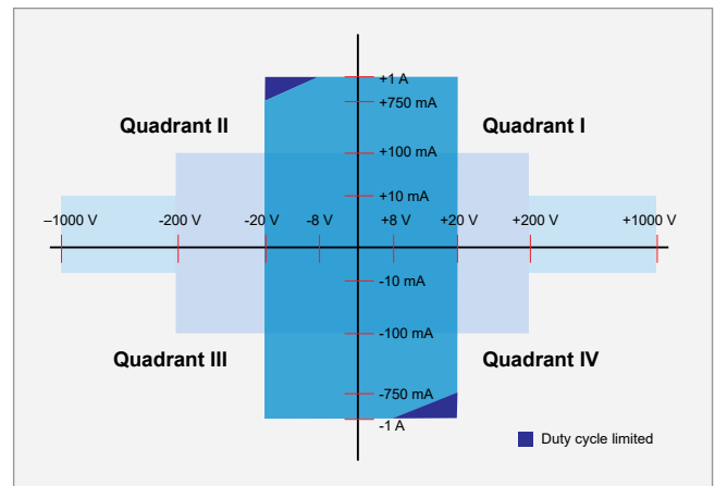
2470 power envelope.
