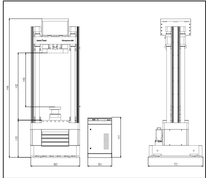
Drawing: Vibrophore 500
