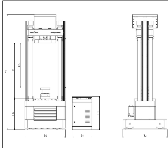
Drawing: Vibrophore 600
