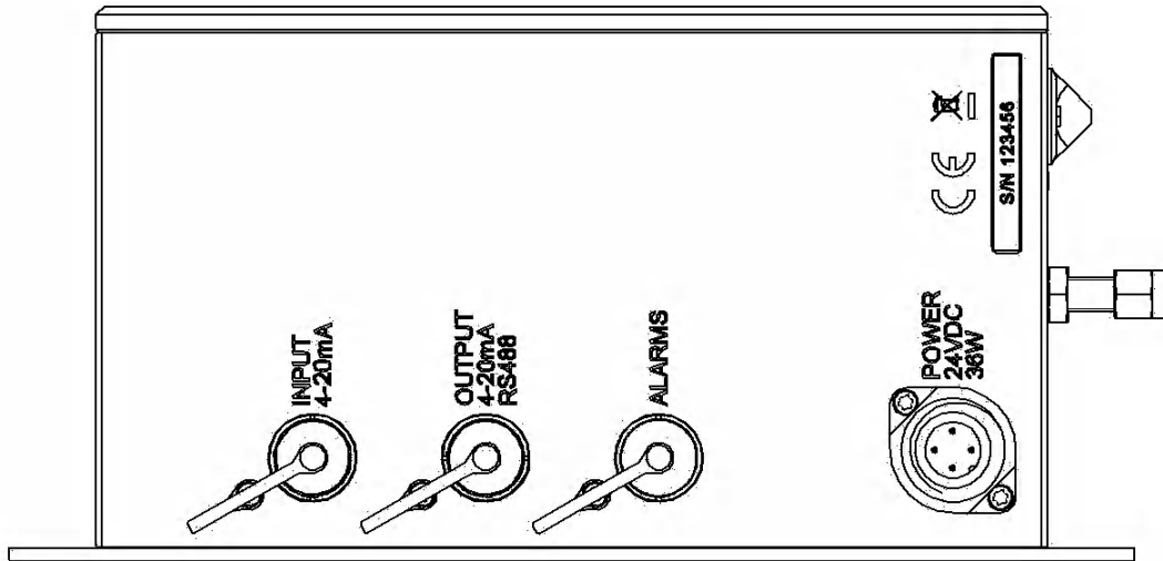
Figure 32 Connections
