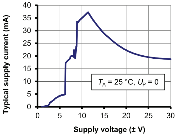
Figure 7: Supply current function of supply voltage
