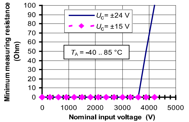
Figure 2: Minimum measuring resistance For T_A under 80\text{ }^\circ\text{C} , the minimum measuring resistance is 0\ \Omega whatever U_C
