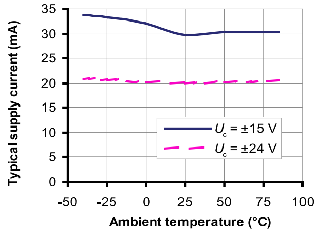
Figure 8: Supply current function of temperature
