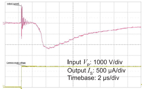
Figure 12: Detail of typical common mode perturbation (4200 V step with 6 kV/µs, R_M = 100 \Omega )
