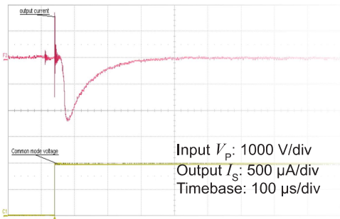
Figure 11: Typical common mode perturbation (4200 V step with 6 kV/µs R_M = 100 \Omega )
