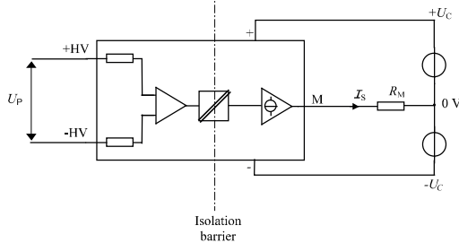
Figure 16: standard characterization schematics for current output transducers ( R_M = 50 \Omega unless otherwise noted)
