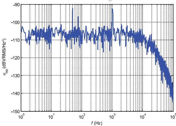
Figure 13: Typical noise power density of U (R_M) with R_M = 50 \Omega
