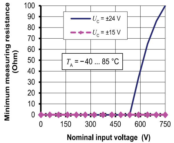
Figure 2: Minimum measuring resistance The derating @ ±24 V is only applicable for T_A = 80 \dots 85^\circ\text{C} For T_A under 80^\circ\text{C} , the minimum measuring resistance is 0 \Omega whatever U_C
