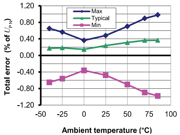
Figure 4: Total error in temperature
