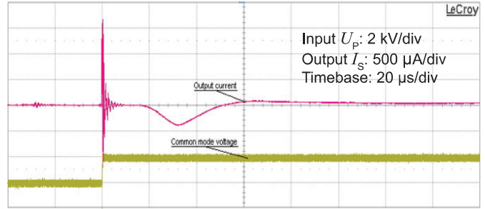
Figure 14: Detail of typical common mode perturbation (2000 V step with 6 kV/μs, R_M = 100 \Omega )
