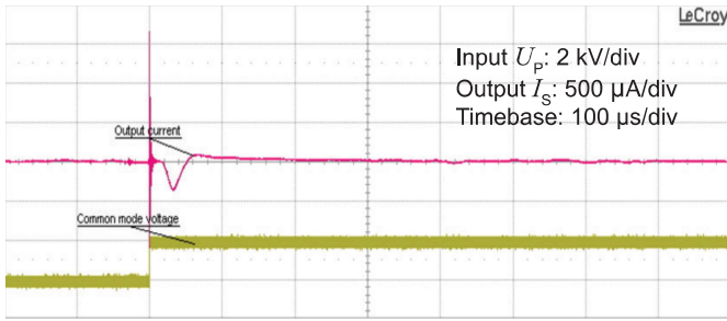
Figure 13: Typical common mode perturbation (2000 V step with 6 kV/μs R_M = 100 \Omega )
