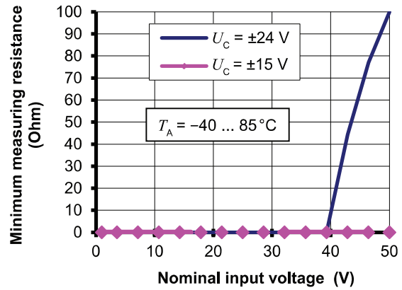
Figure 2: Minimum measuring resistance For T_A under 80 °C, the minimum measuring resistance is 0 Ω whatever U_C
