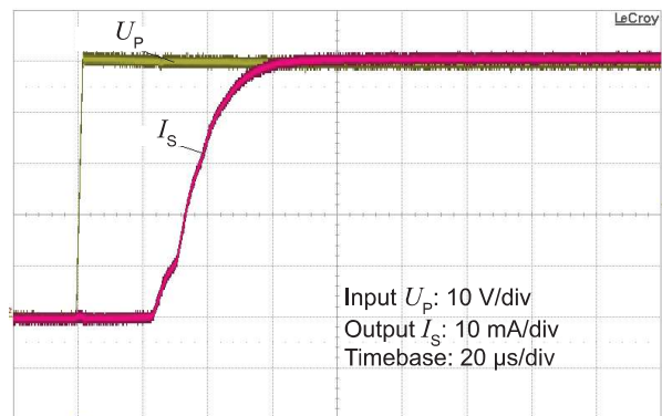
Figure 6: Typical step response (0 to 50 V)
