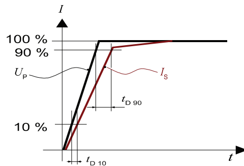
Figure 19: Delay time t_{D90} @ 90 and delay time t_{D10} @ 10
