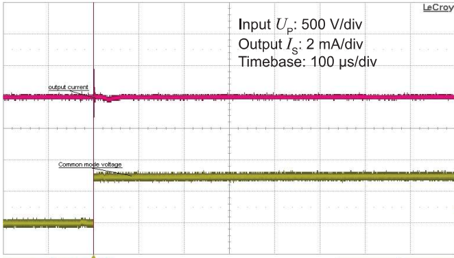
Figure 13: Typical common mode perturbation (750 V step with 6 kV/µs, R_M = 100 \Omega )
