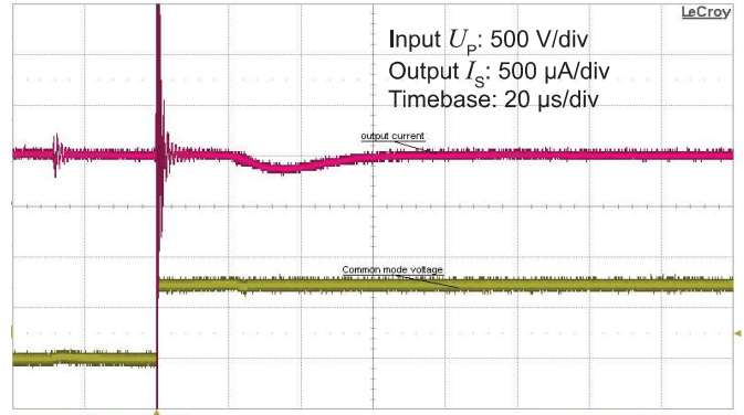
Figure 14: Detail of typical common mode perturbation (750 V step with 6 kV/µs, R_M = 100 \Omega )
