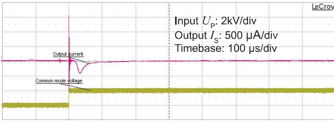
Figure 13: Typical common mode perturbation (125 V step with 6 kV/µs R_M = 100 \Omega )
