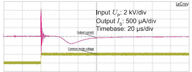
Figure 14: Detail of typical common mode perturbation (125 V step with 6 kV/µs, R_M = 100 \Omega )
