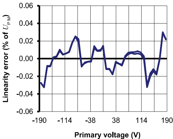
Figure 17: Typical linearity error at 25 °C
