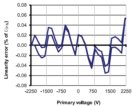
Figure 7: Typical linearity error at 25 °C
