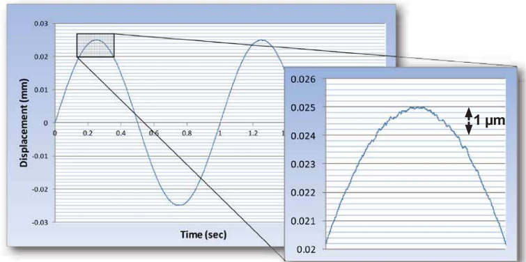
50 µm peak-to-peak waveform with an ElectroForce® Series II 3200 Test Instrument
