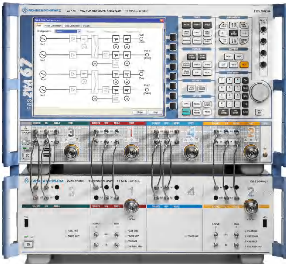
Setup for S-parameter, harmonic, intermodulation and pulsed measurements.
