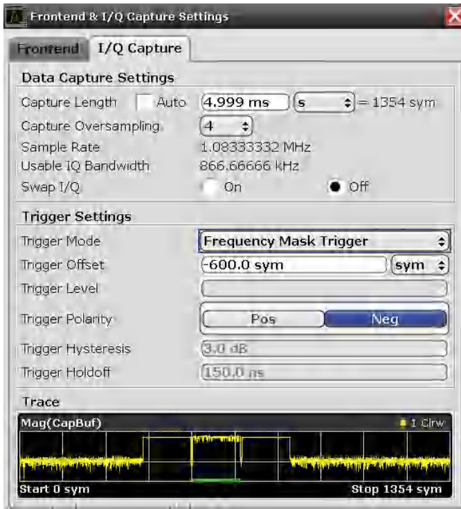
Definition window for I/Q data capturing in the R&S®FSV-K70 general vector signal analysis option: The FMT trigger mode is available in addition to the standard trigger modes.
