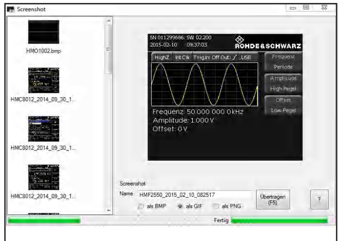
Abb. 5.15: Screenshot-Modul
