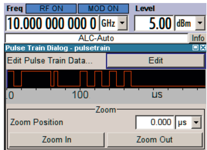
Diagram of the pulse train
