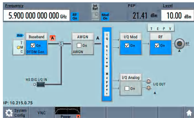
Functional block diagram of the R&S®SMBV100B
