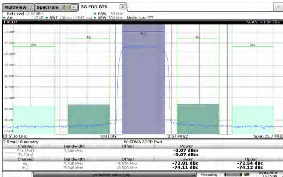
Measured ACPR for WCDMA test model 1, 64 DPCH
