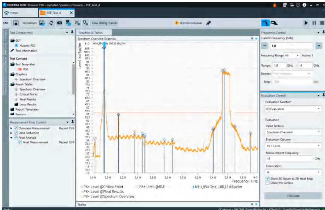
RSE measurement of a 5G FR1 NSA device with the 4G and 5G carrier present.
