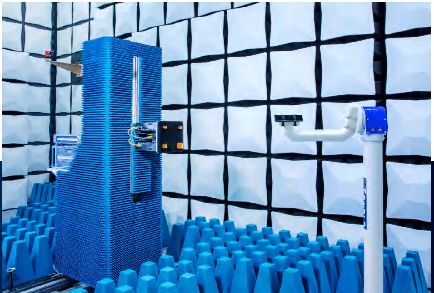
R&S®TS8996 setup for frequencies above 41 GHz with automatic positioner for frequency and polarization change.
