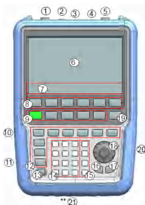
Figure 3-4: Front panel of R&S Spectrum Rider
