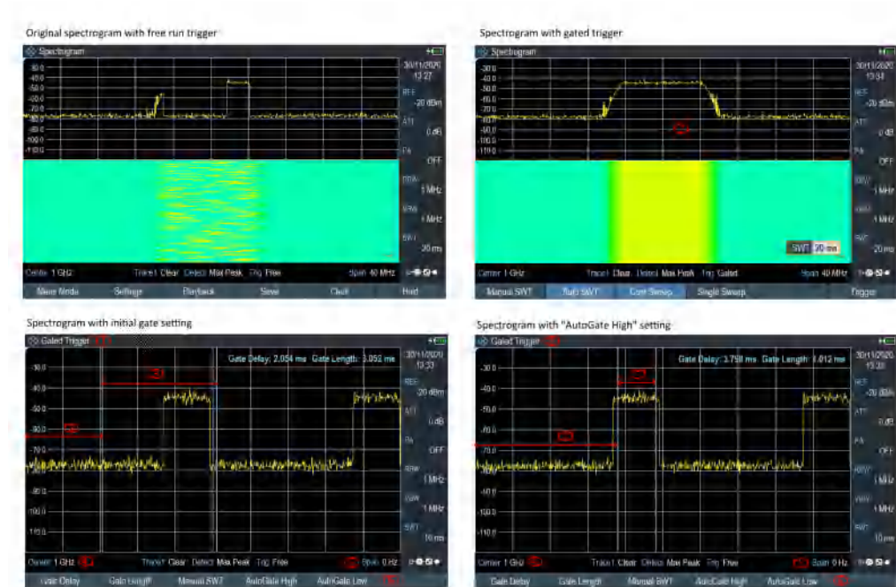
Figure 6-12: Gated trigger measurement
