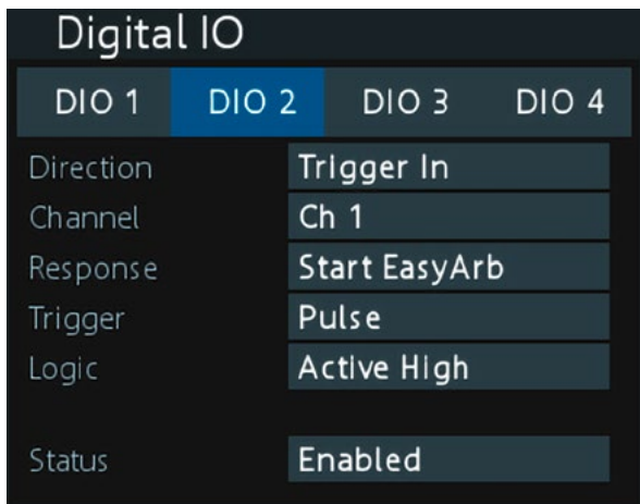
Here, channel 1 of the optional digital I/O interface (R&S®NGE-K103) is used as a trigger input
