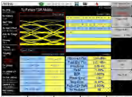
PTC ACSES Receiver Test Signal Generator
