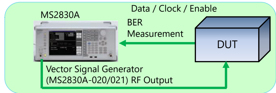
BER Measurement Setup Example (with MS2830A-020/021 installed)
