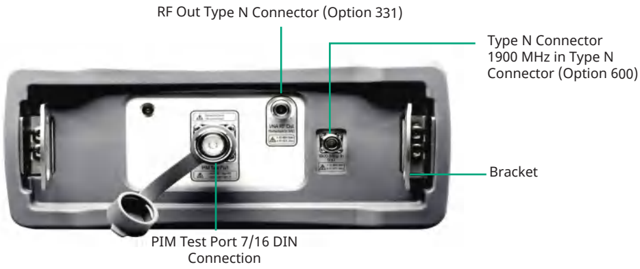
Single Port Instruments RF Connector Configuration
