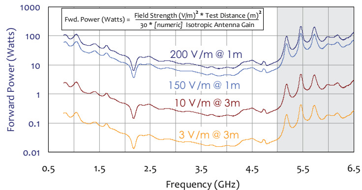
Figure 9 – Power requirements for various fields strengths/distances
