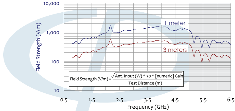
Figure 8 – Calculated Field Strength with 450W input power
