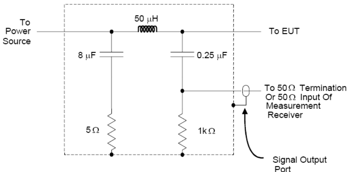
Figure 1 – Example of an equivalent LISN circuit
