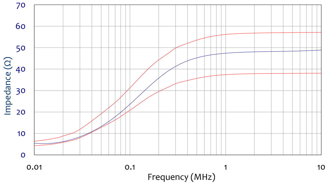
Figure 2 - Impedance (AE Port: Open ) compared to Mil-Std 461 requirements.
