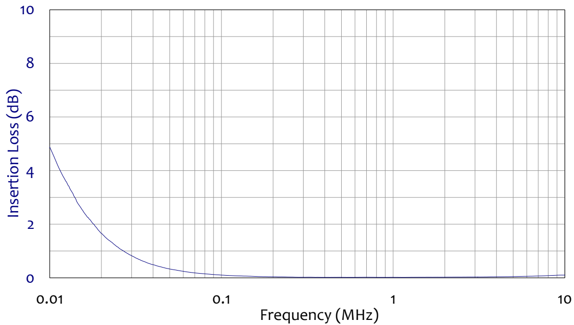
Figure 3 – Insertion Loss
