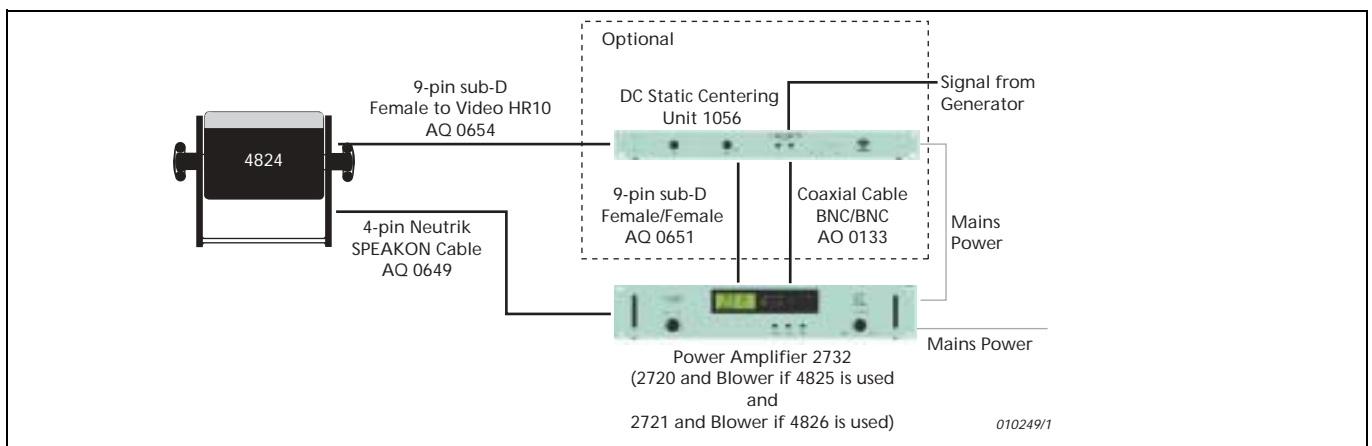
Fig. 1 DC Static Centering Unit setup when used with Modal Exciter Types 4824, 4825 and 4826
