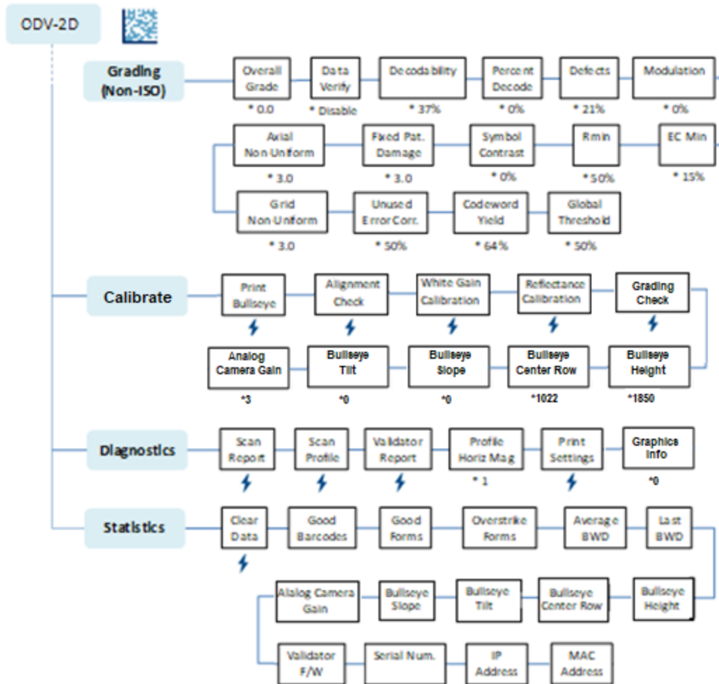
Figure 3 Validator Section and Submenus, Continued
