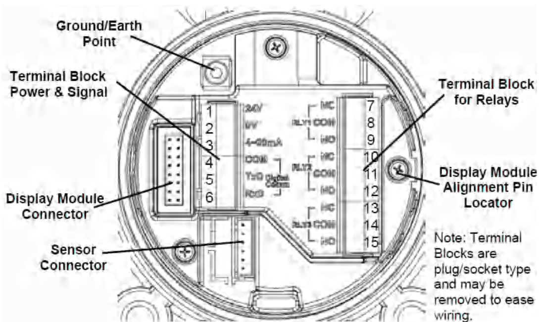
Diagram 9 Terminal module
