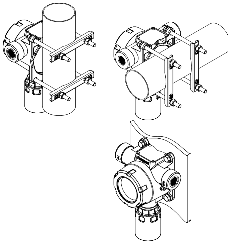
Diagram 5 Mounting arrangements
