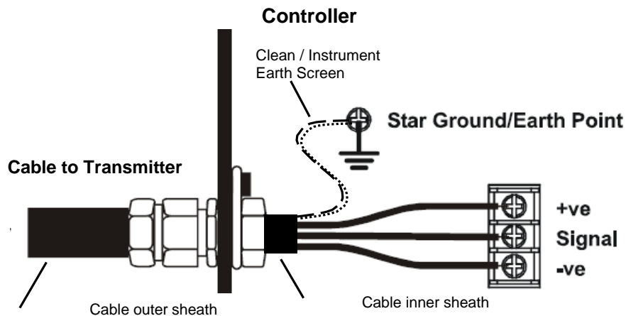
Diagram 11 Controller Grounding
